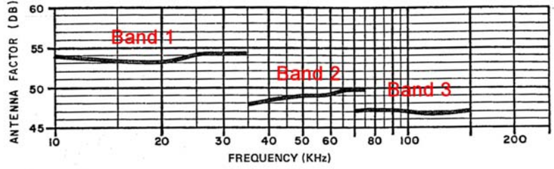
ANTENNA FACTOR CHART RVR-25 (TYPICAL)
