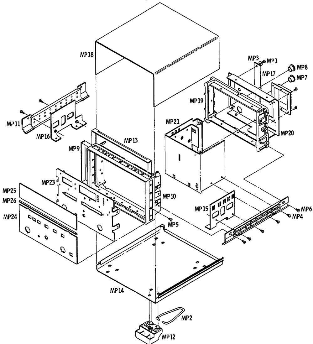
Figure 6-1. Cabinet Parts
