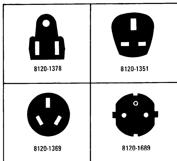
Figure 2-2. Power Cable and Mains Plug Part Numbers
